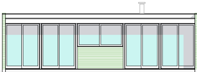
Bedroom Elevation
